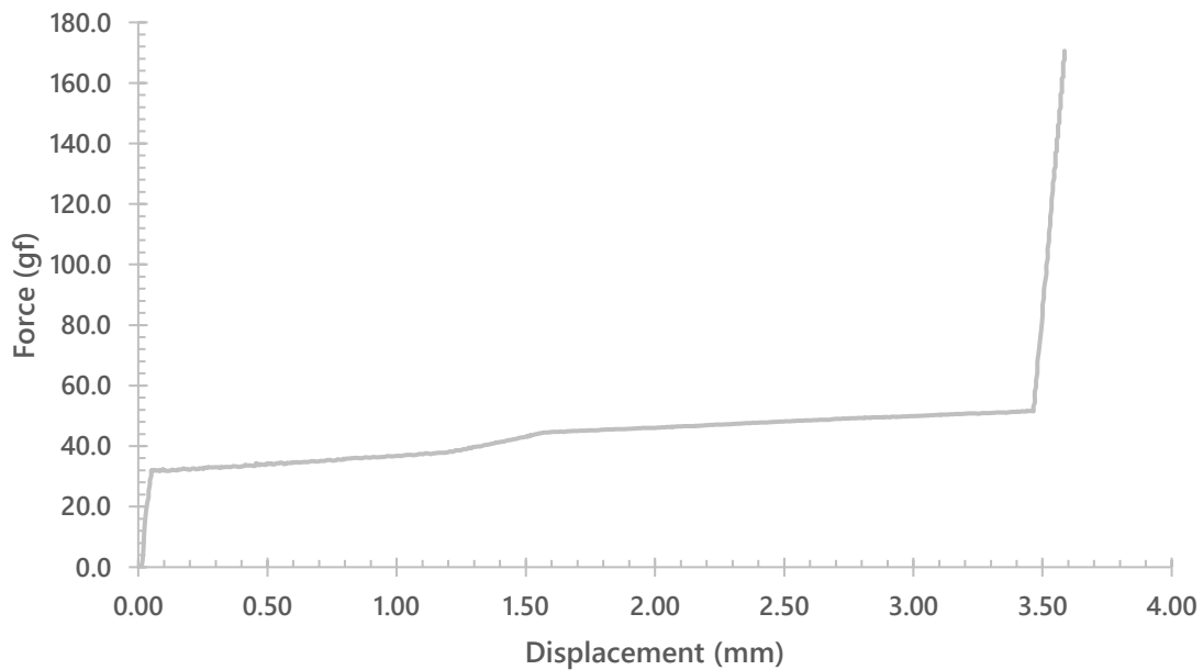
KTT Lightning V2 (Upstroke)
